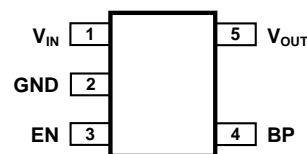
5-Pin Plastic SOT-23-5 Surface Mount (Top View)
