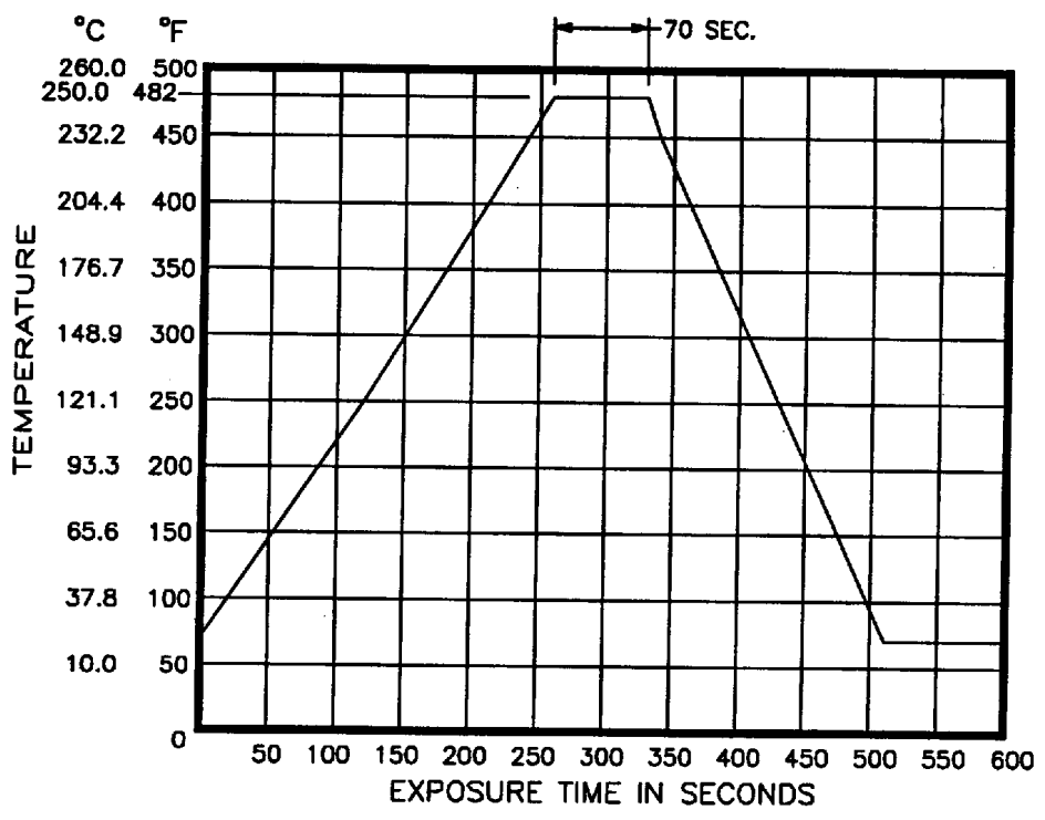
FIGURE 30: Maximum Recommended Re-Flow Profile
