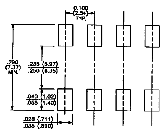
FIGURE 29: Recommended footprint, 8-pin J-Style.
