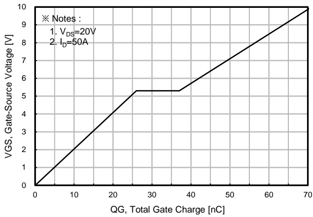
Fig. 7. Gate Charge
