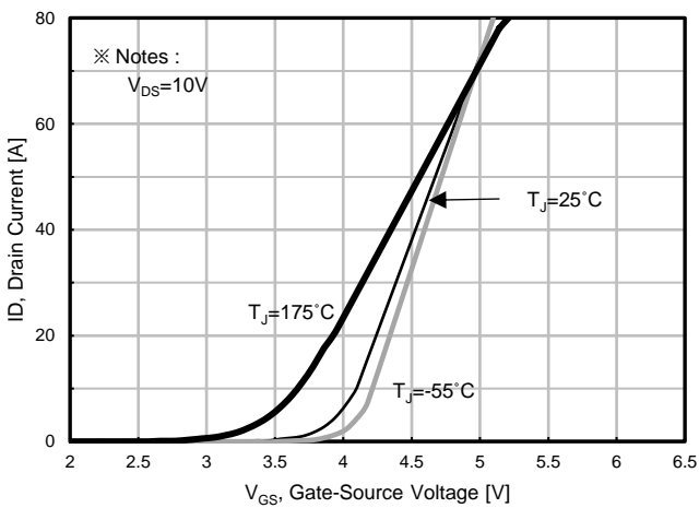
Fig. 5. Transfer Characteristics
