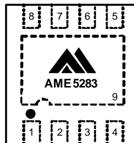
DFN-8C (3mmx3mmx0.75mm) Top View
