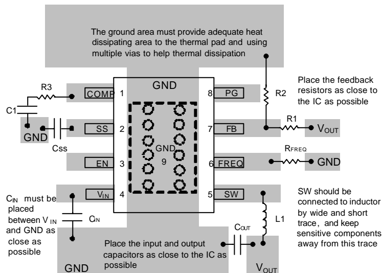
Figure 3. AME5283 Regulators Layout Diagram
