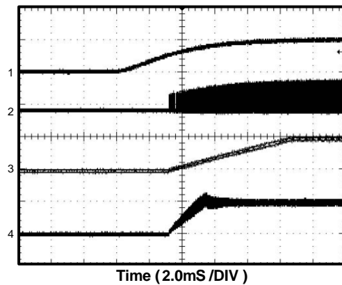
Power ON from V_{IN}
