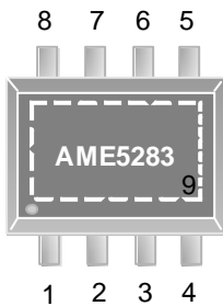
SOP-8/PP Top View
