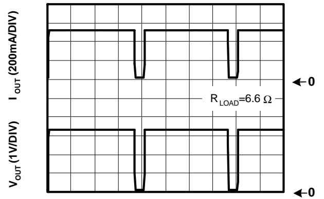
Overtemperature Shutdown
