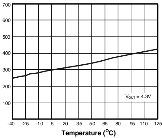
Dropout Voltage
