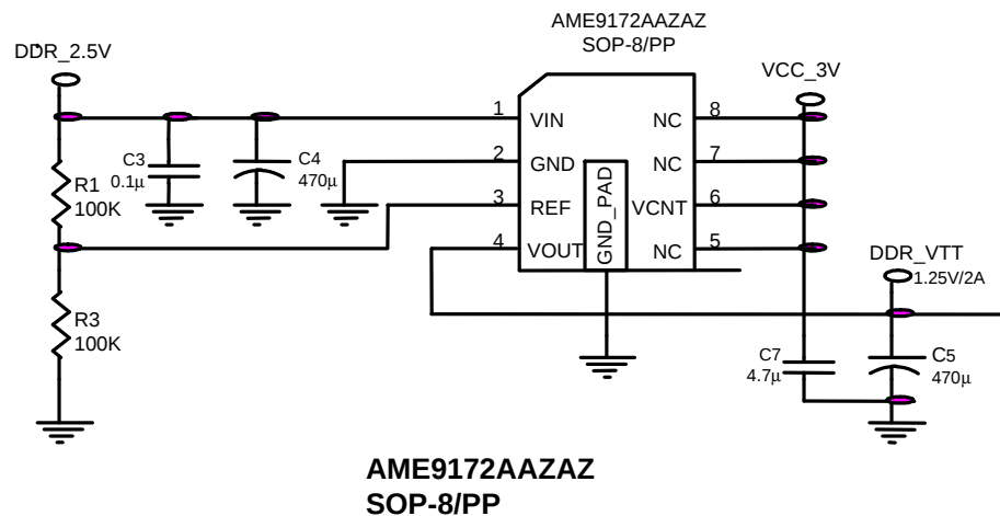
Fig 2 : Application Circuit AME9172AAZAZ
