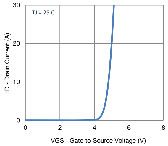
2. Transfer Characteristics
