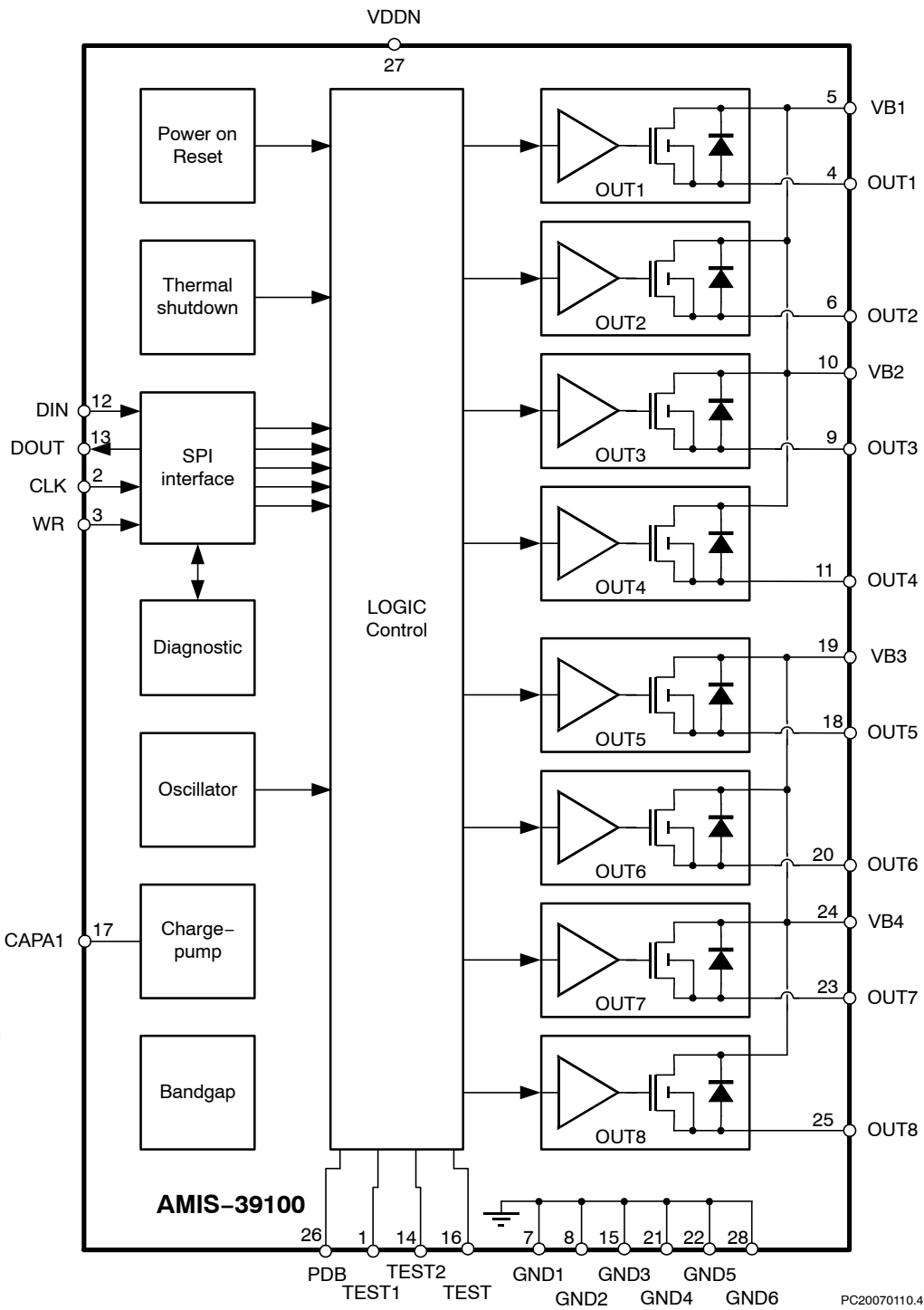
Figure 1. Block Diagram
