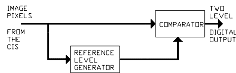
ANALOG SIGNAL REFERENCE GENERATOR AND A SINGLE BIT COMPARATOR FIGURE 3
