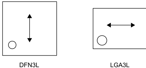
Figure 2. Sensing direction
