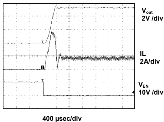
Start-Up Response
