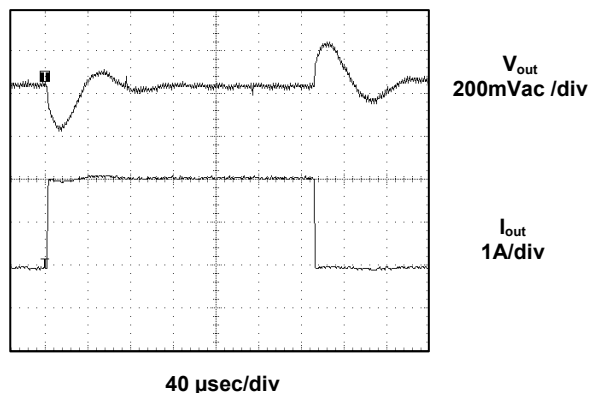
Load Transient 1A to 3A, V_{out} = 5V , V_{in} = 12V
