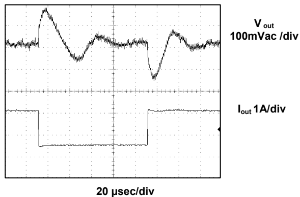
Load Transient 500mA to 2A, V_{out} = 5V , V_{in} = 12V
