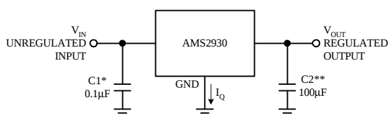
AMS2930-X (Fixed Output)
