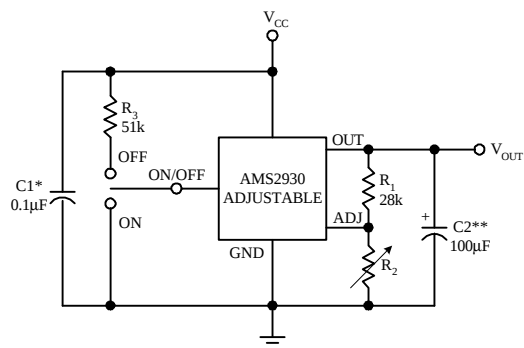
AMS2930C (Adjustable Output)
