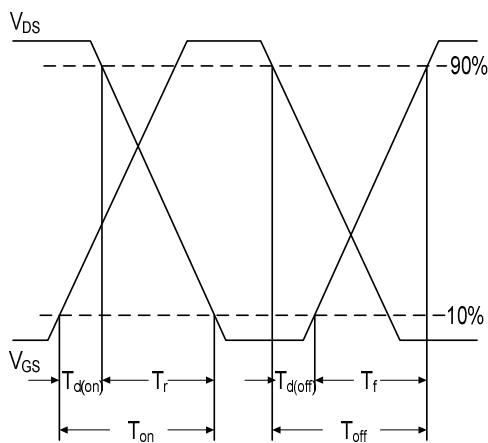
Fig.10 Switching Time Waveform
