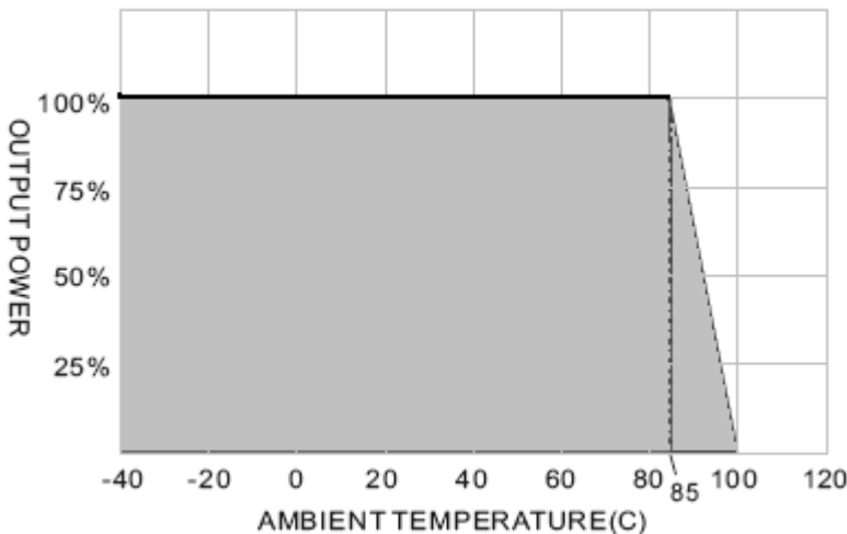
Derating Curve
