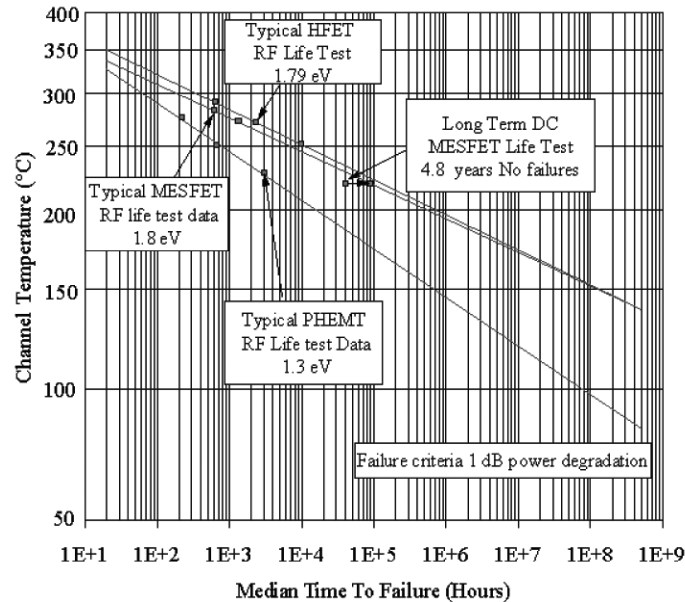
Figure 2. Typical MTTF data for TriQuint MESFET, HFET, and PHEMT.
