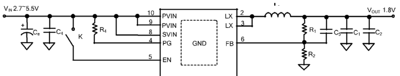
Figure 1. Schematic Diagram
