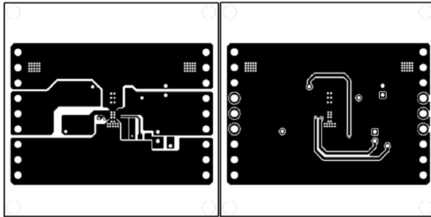
(a) (b) Figure 4. PCB Layout Plots: (a) top layer, (b) bottom layer
