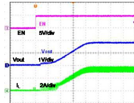
Time (200us/div)
