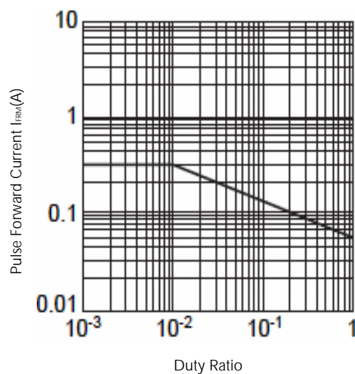
Duty Ratio vs. Pulse Forward Current Condition : T_a = 25^\circ\text{C} , t_w = 100\mu\text{s}
