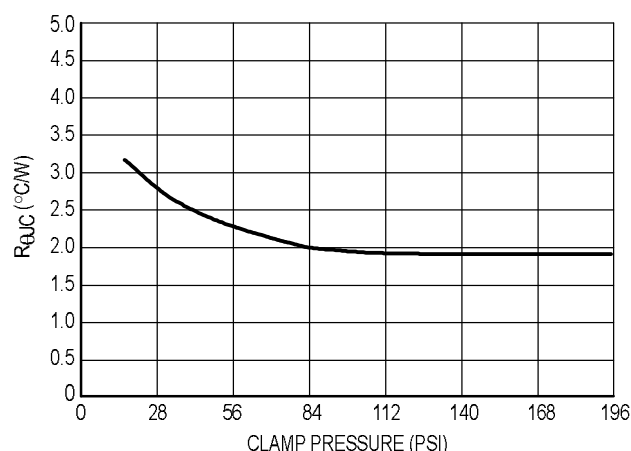
Figure 4. R_{\theta JC} versus Clamp Pressure
