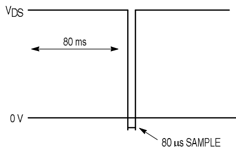
Figure 3. Example of a Power and Sample Pulse Train During R_{\theta JC} Measurement of a TMO5 Device
