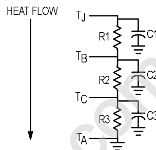
Figure 1. Thermal Electrical Equivalent Circuit
