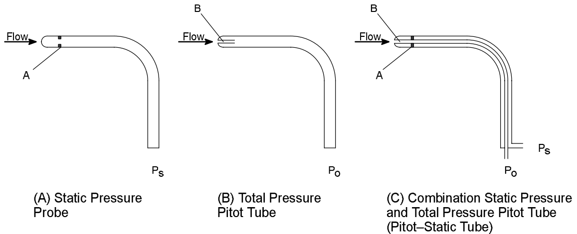
Figure 6. Types of Pressure Probes
