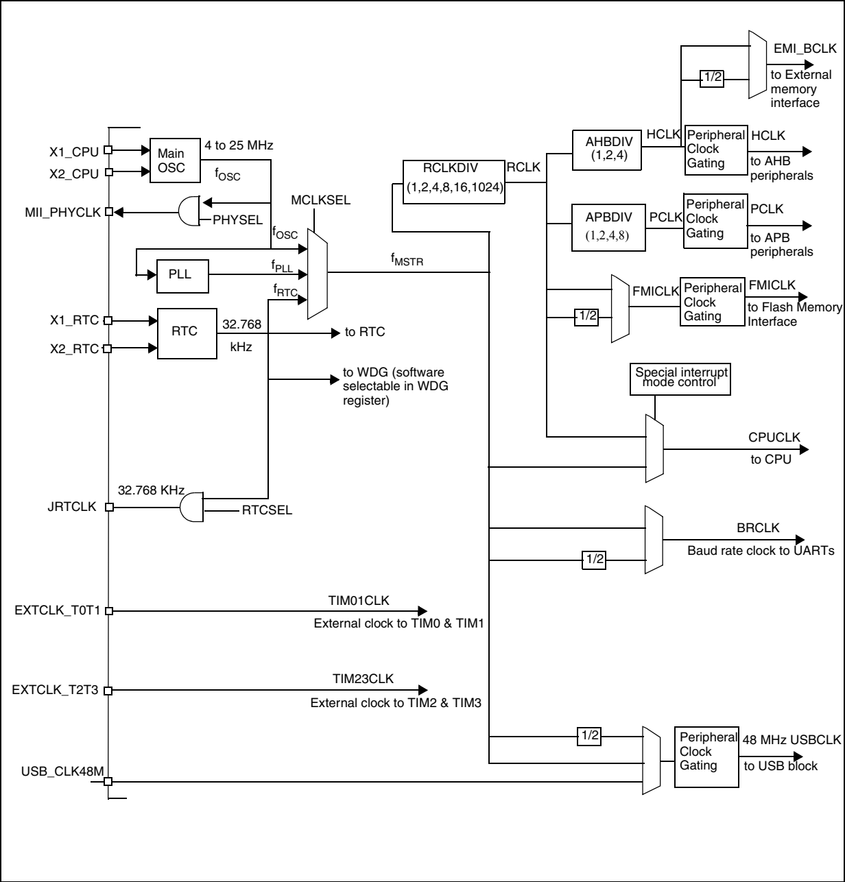
Figure 2. Clock control
