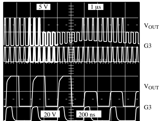
Figure 16. Composite Sample-and-Hold Output and the Gate 3 Control Signal
