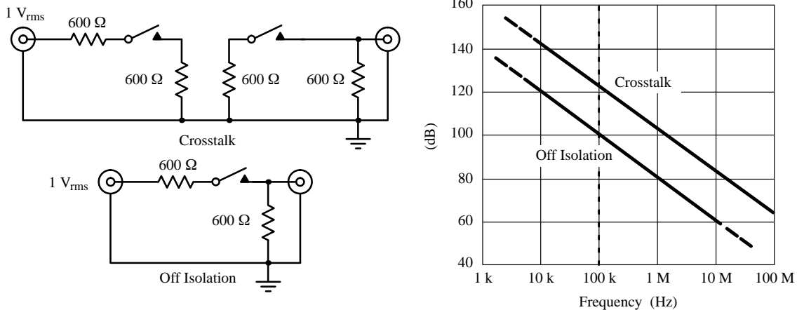
Figure 11. SD5000 Crosstalk and Off-Isolation vs Frequency
