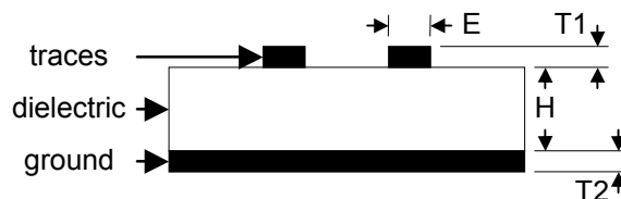
Figure 3. Side View of Printed Circuit Board
