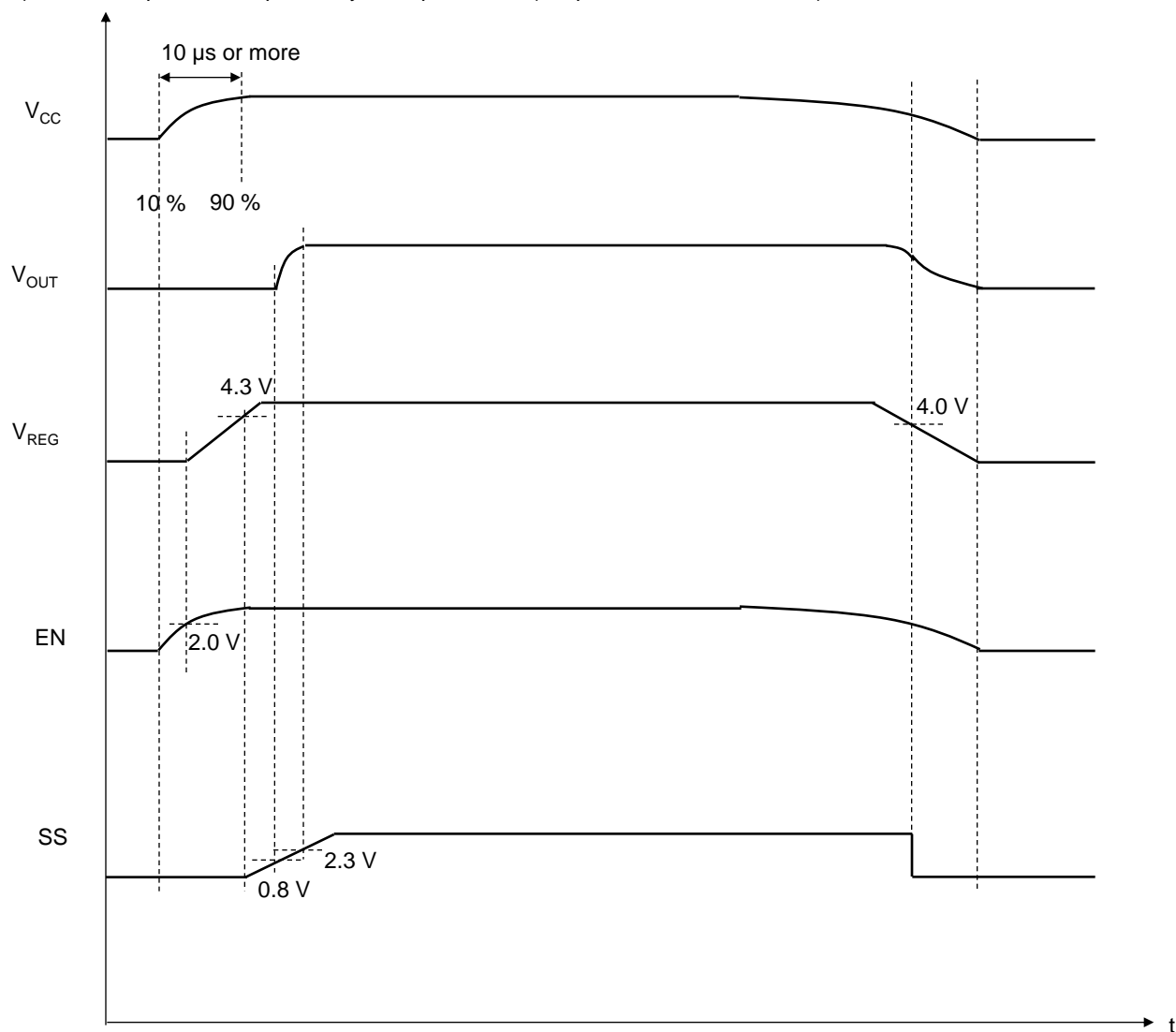
Figure : Power ON/OFF Timing (2)
