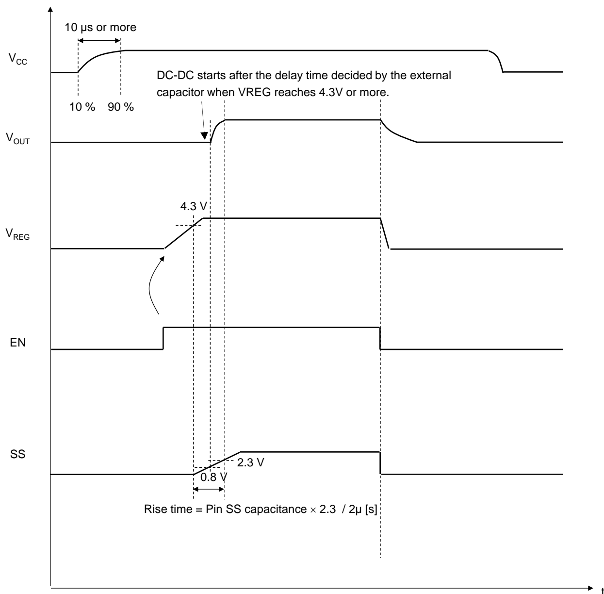
Figure : Power ON/OFF sequence by EN
