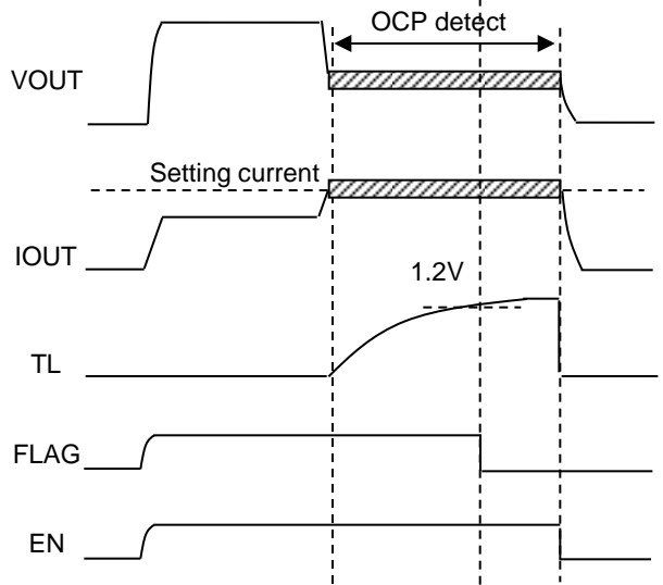
Figure : Method of detection of Over-Current Protection function
