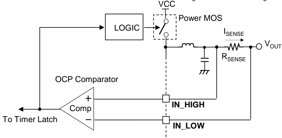
Figure : Over-Current Protection circuit block diagram
