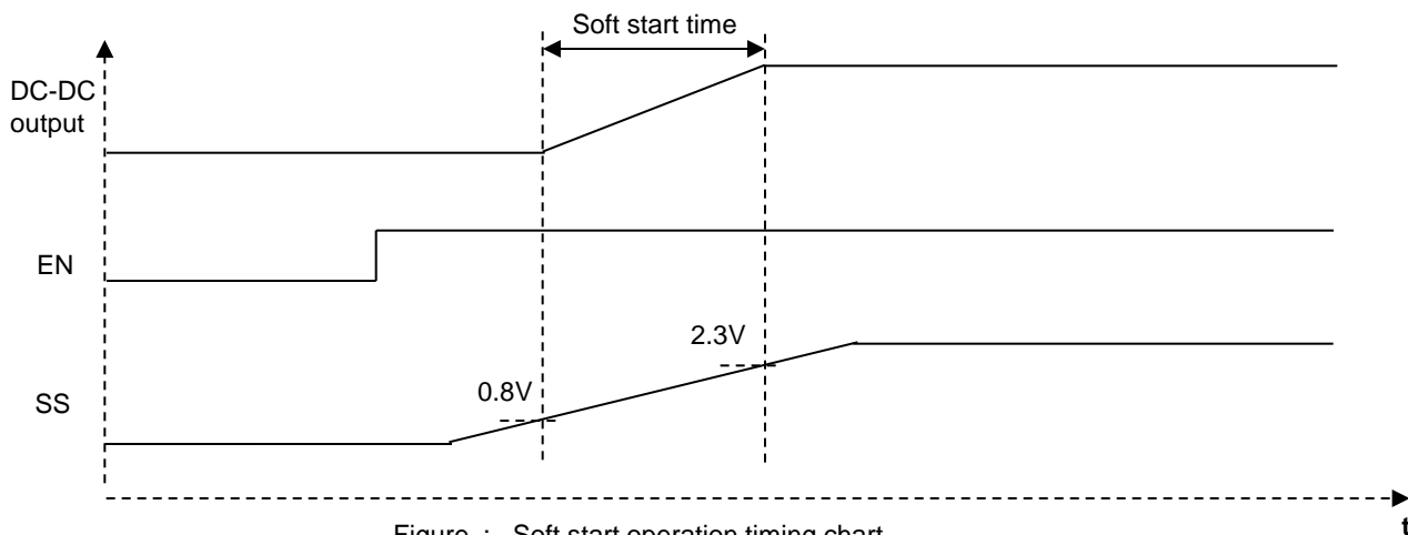
Figure : Soft start operation timing chart
