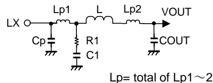
Figure : Snubber circuit value
