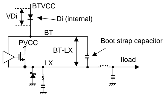
Figure : Boot Strap external circuit
