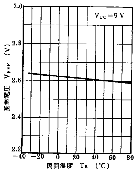
V_{REF} - T_a
