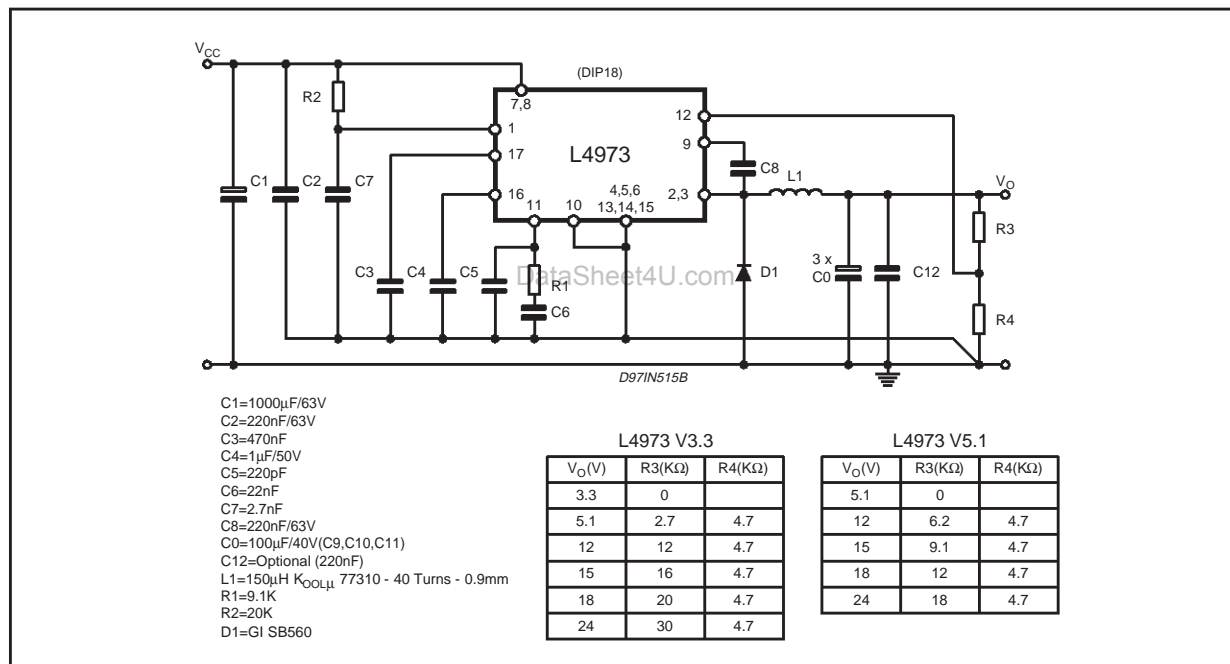
Figure 19. Application circuit
