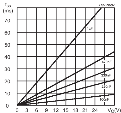
Figure 13. Soft start time vs. V O and C SS
