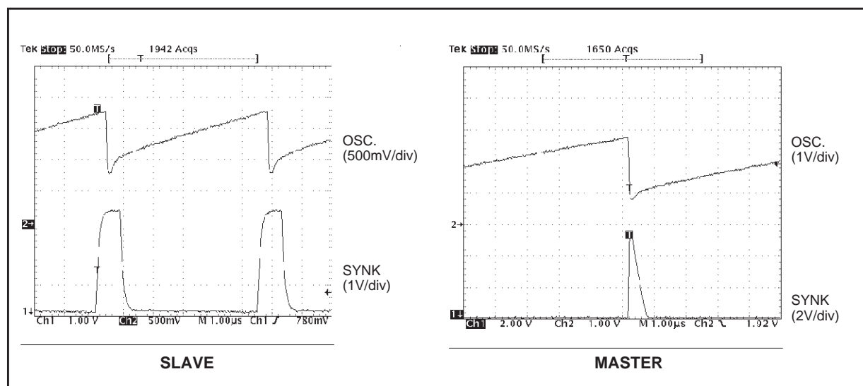
Fig. 17 shows the typical synchronization waveforms when the device is used as slave and as master.
