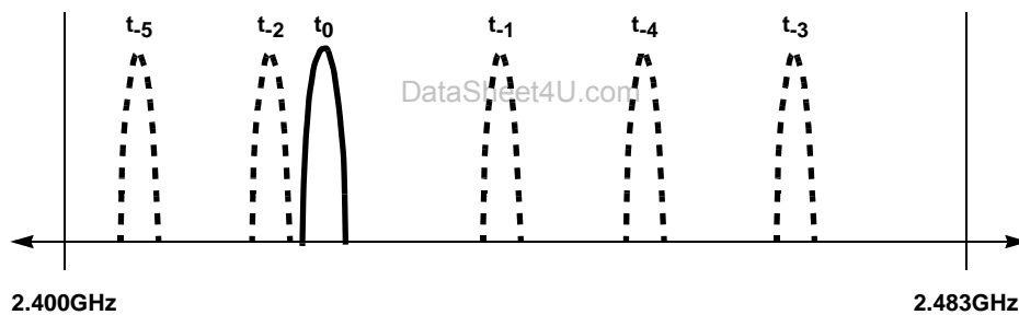
FIGURE 6. FHSS RADIOS HOP CHANNELS IN A PSEUDO RANDOM SEQUENCE
