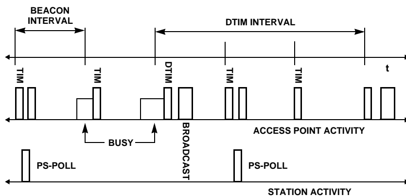
FIGURE 9. TIMING BEACONS FACILITATE POWER SAVING MODE
