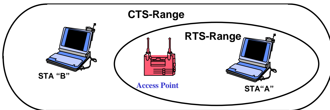
FIGURE 8. RTS/CTS PROCEDURE ELIMINATES THE "HIDDEN NODE" PROBLEM
