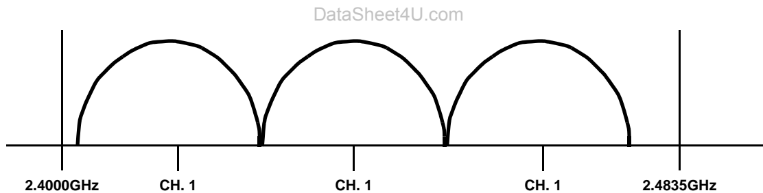
FIGURE 5. THREE NON-OVERLAPPING DSSS CHANNELS IN THE ISM BAND
