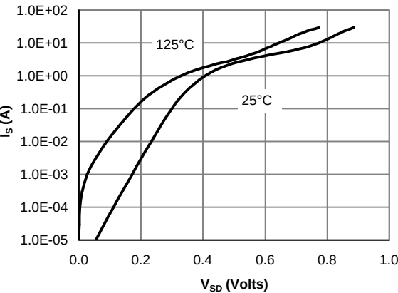
Figure 6: Body-Diode Characteristics
