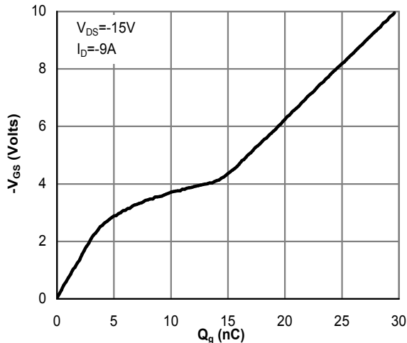
Figure 7: Gate-Charge Characteristics
