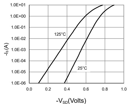
Figure 6: Body-Diode Characteristics
