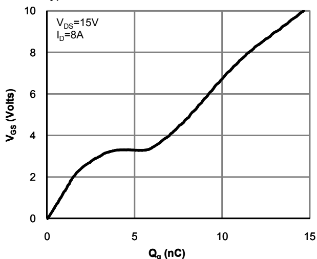
Figure 7: Gate-Charge Characteristics
