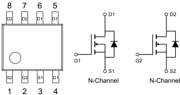
SOP-8
