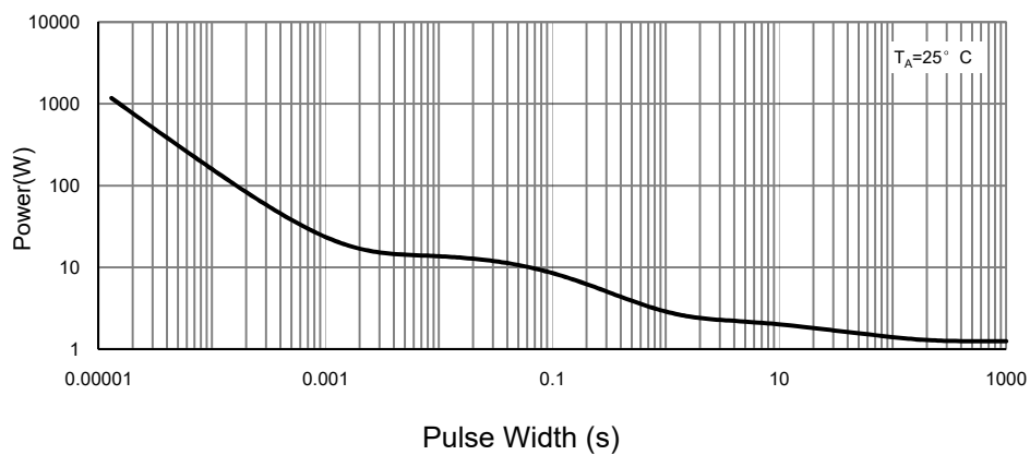
Figure 11: Single Pulse Power Rating Junction-to-Ambient (Note F)
