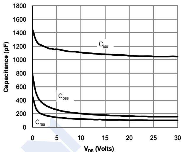
Figure 8: Capacitance Characteristics
