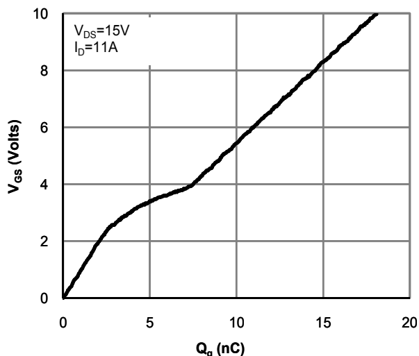
Figure 7: Gate-Charge Characteristics
