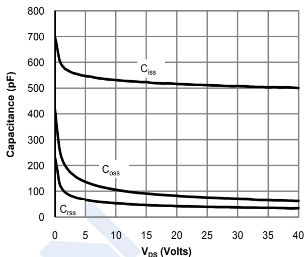
Figure 8: Capacitance Characteristics
