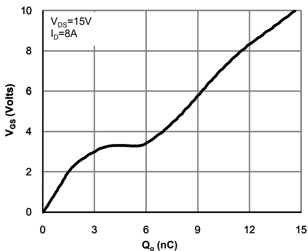
Figure 7: Gate-Charge Characteristics
