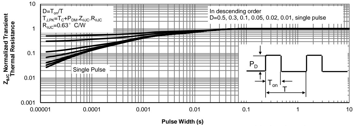
Figure 16: Normalized Maximum Transient Thermal Impedance for AOT(B)11S65L (Note F)
