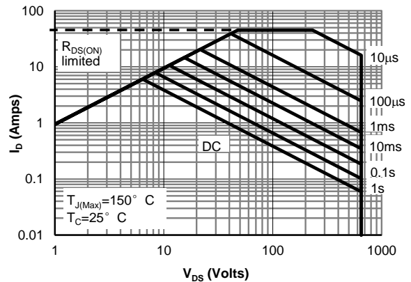
Figure 12: Maximum Forward Biased Safe Operating Area for AOTF11S65 (Note F)
