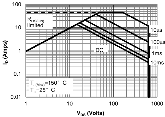
Figure 11: Maximum Forward Biased Safe Operating Area for AOT(B)11S65L (Note F)
