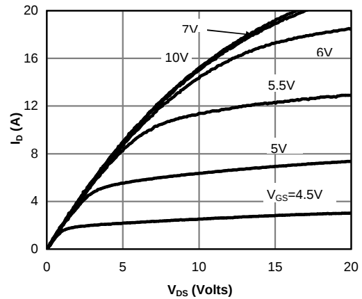
Figure 2: On-Region Characteristics@125°C
