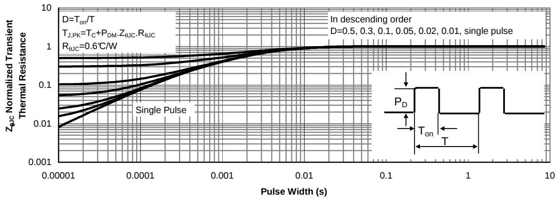
Figure 16: Normalized Maximum Transient Thermal Impedance for AOT(B)15S65 (Note F)
