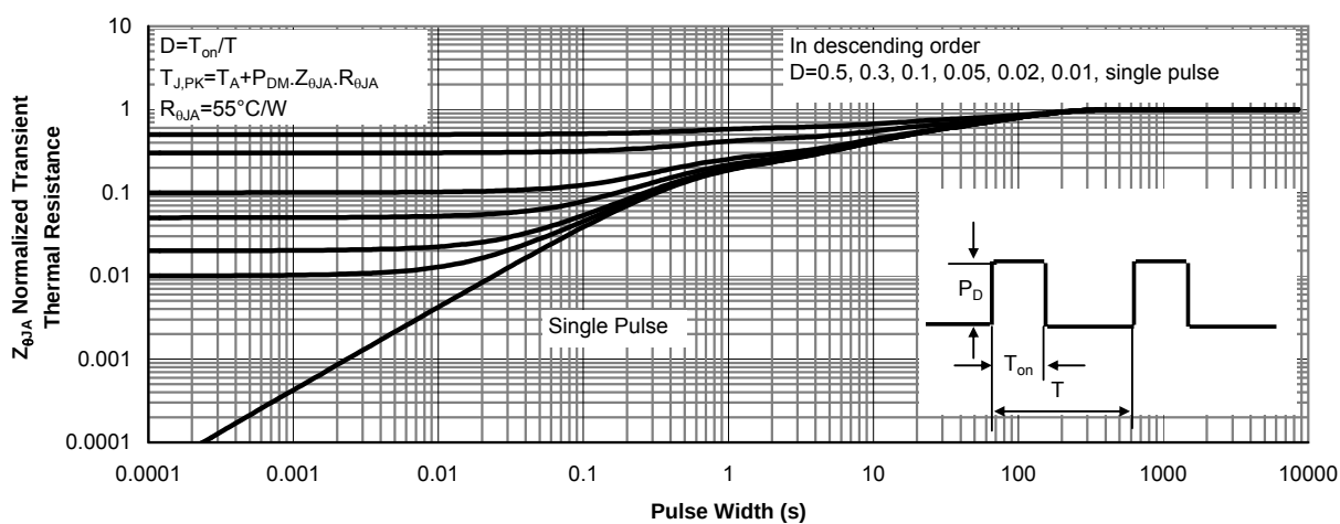
Figure 15: Normalized Maximum Transient Thermal Impedance (Note G)
