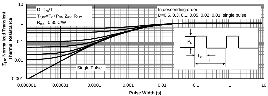
Figure 14: Normalized Maximum Transient Thermal Impedance for AOK27S60 (Note F)
