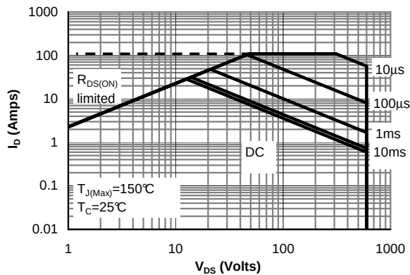
Figure 11: Maximum Forward Biased Safe Operating Area for AOK27S60 (Note F)
