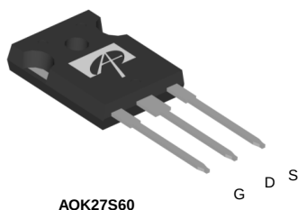
Top View TO-247
