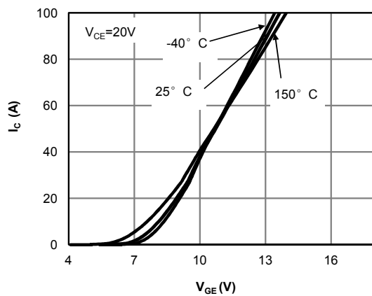
Figure 3: Transfer Characteristic
