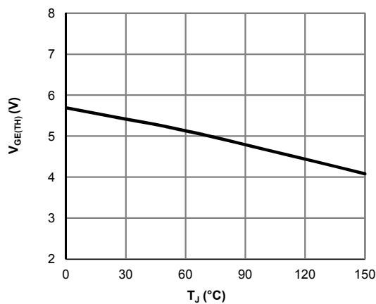
Figure 5: V_{GE(TH)} vs. T_j
