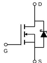
SRFET™ Soft Recovery MOSFET: Integrated Schottky Diode
