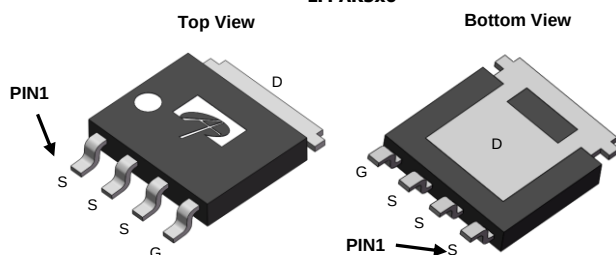
LFPAK5x6
