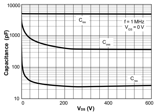
Figure 10. Capacitance Characteristics
