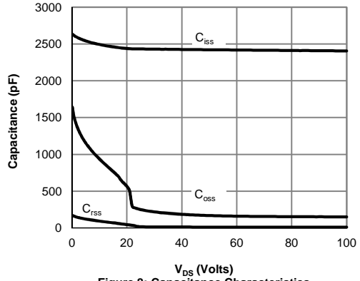
Figure 8: Capacitance Characteristics
