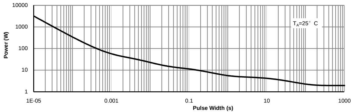
Figure 14: Single Pulse Power Rating Junction-to-Ambient (Note H)
