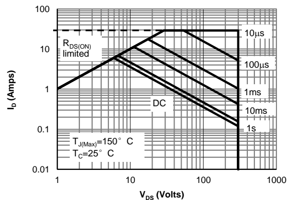
Figure 10: Maximum Forward Biased Safe Operating Area for AOTF12N30 (Note F)
