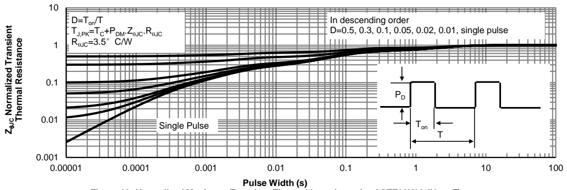
Figure 13: Normalized Maximum Transient Thermal Impedance for AOTF12N30 (Note F)
