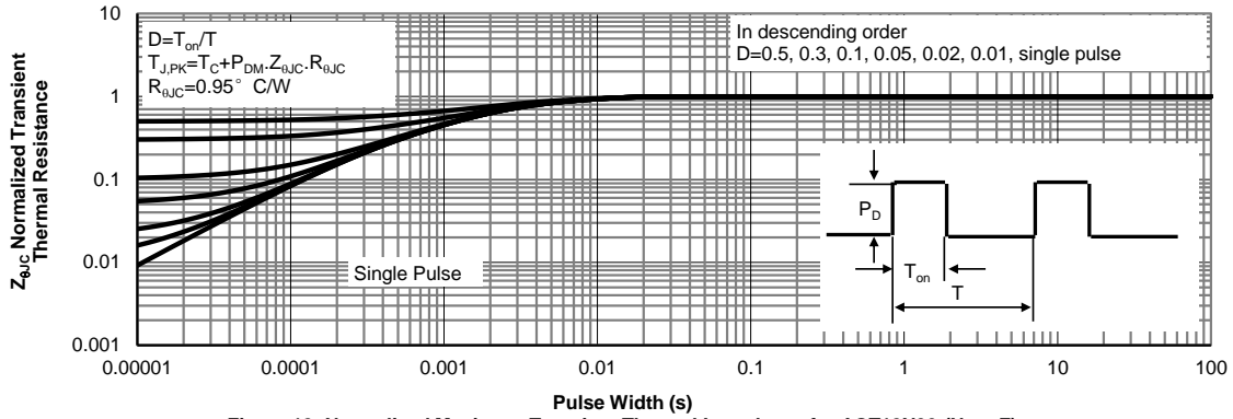
Figure 12: Normalized Maximum Transient Thermal Impedance for AOT12N30 (Note F)
