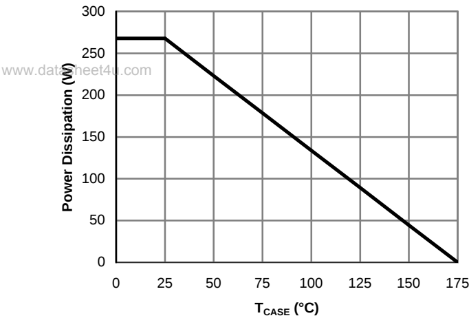
Figure 12: Power De-rating (Note B)
