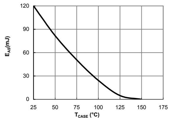
Figure 12: Avalanche energy
